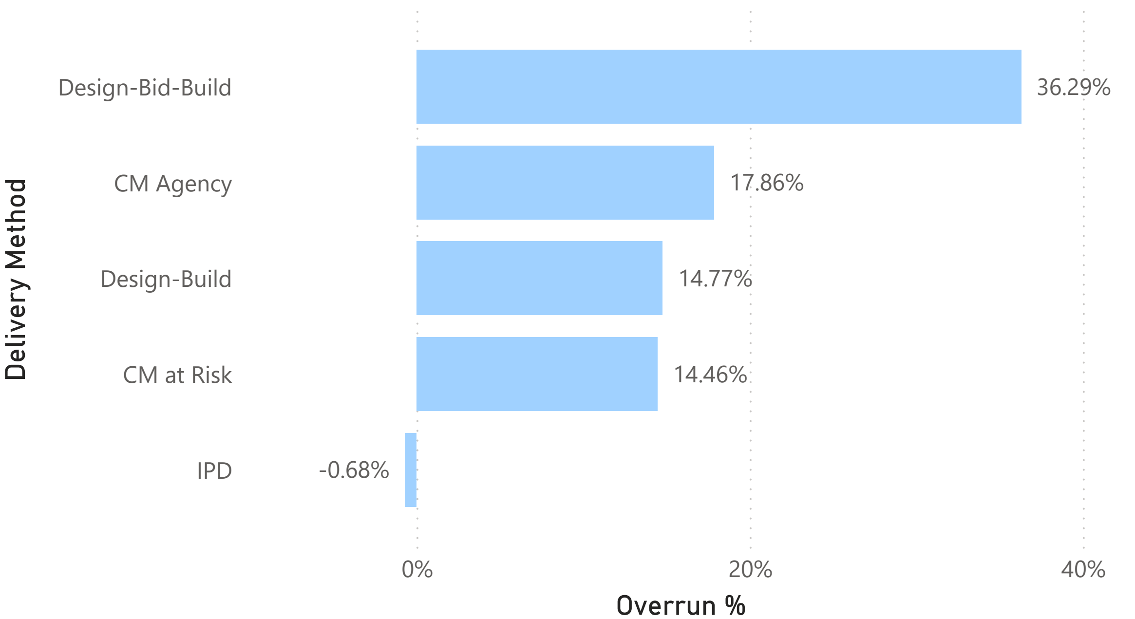
Cost Overrun by Delivery Method
